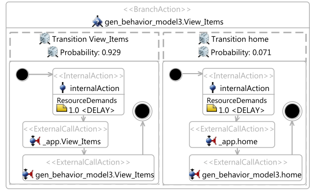
Figure 2: Generated RDSEFF example
