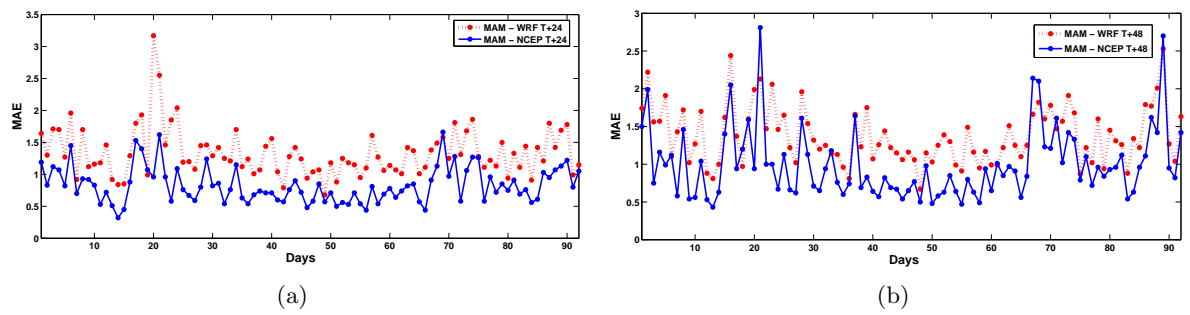
Fig. 2. MAE (Mean Absolute Error) for WRF and NCEP 24 (a) and 48 (b) hour forecasts for wind speed at 10 meters valid for MAM period
