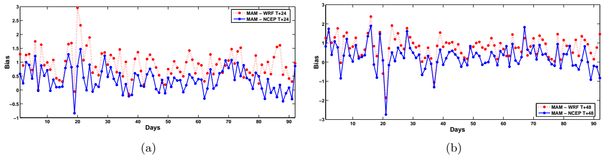
Fig. 1. Bias (Mean Error) for WRF and NCEP 24 (a) and 48 (b) hour forecasts for wind speed at 10 meters valid for MAM period
