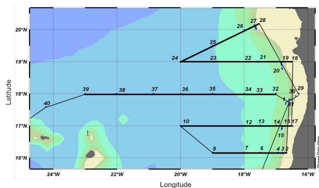
Fig. 1. Cruise track and locations of the sampling stations during the ATA-03 cruise in February 2008. Bold black lines indicate the onshore-offshore transects. The colour coding represents the bathymetry of the sampling area. Dark blue to light brown indicate deep waters (3600 m) to shallow waters (50 m).
