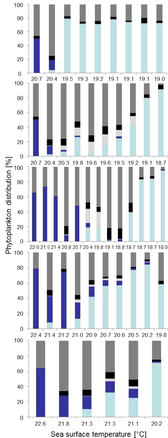
Fig. 3. Phytoplankton distribution in percentage based on their group specific chlorophyll concentration calculated by using the CHEMTAX® program: diatoms (light blue), cyanobacteria (dark blue), dinoflagellates (light grey), haptophytes (black) and other groups (including cryptophytes, chlorophytes, pelagophytes, dark grey) in 5 m depth along onshore-offshore transects between 16^{\circ} (lowest panel) and 20^{\circ}\text{N} (upper panel).
