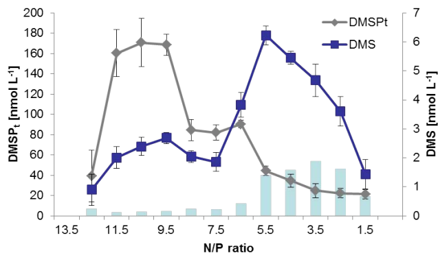
Fig. 6. N:P ratio vs. \text{DMSP}_t (grey diamonds) and DMS (blue squares) at 5 m depth. N stands for the sum of dissolved nitrate and nitrite, and P stands for phosphate. Blue bars show DMS: \text{DMSP}_t ratios.
